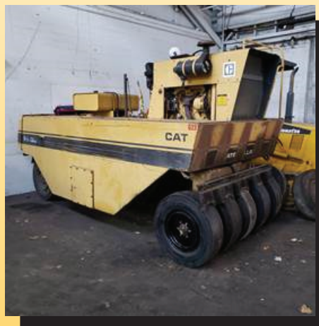
Pneumatic tire roller, 1987 Caterpillar PS-130
